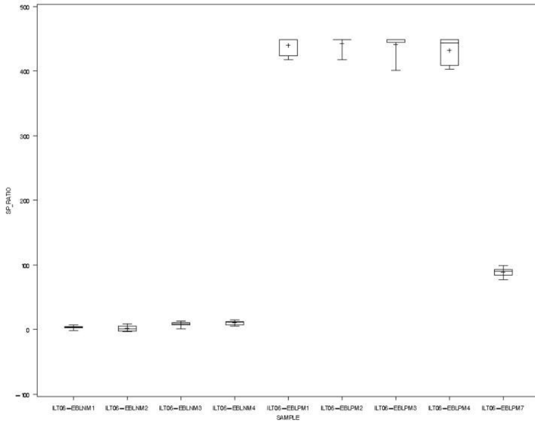
boxplot for each SAMPLE grouped by LABNR LABNR=4
