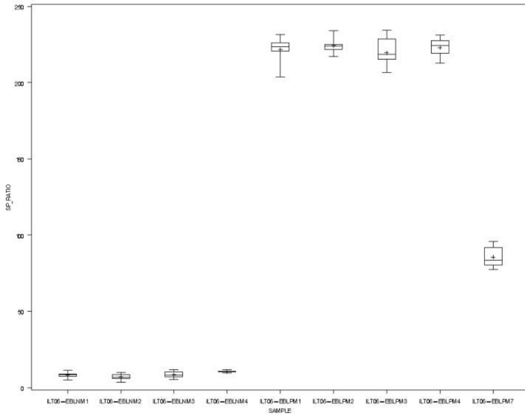
boxplot for each SAMPLE grouped by LABNR LABNR=2
